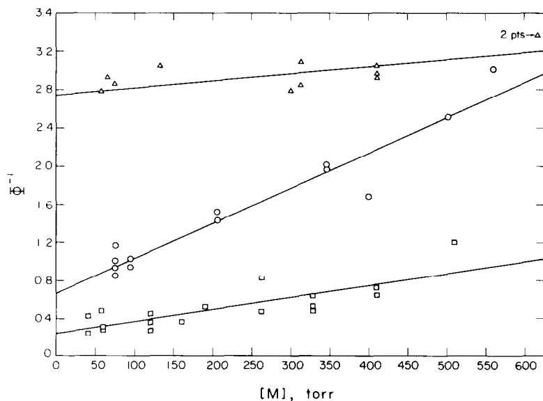
Fig. 4. Plots of \Phi^{-1} vs. [M] where [M] = [\text{air}] + 3[\text{CH}_3\text{CHO}] : \circ , 310.5 nm; \square , 302.0 nm; \triangle , 294.0 nm. The data at 302.0 nm have been displaced downward by 0.5, and those at 294.0 nm have been displaced upward by 2.0 for clarity.
