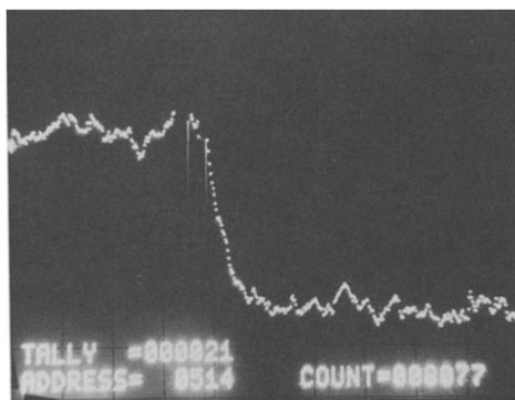
Fig. 2. Plot of light intensity at 250.5 nm vs. time after the flash in the 310.5 nm photolysis of a mixture containing \text{Cl}_2 at 3.4 Torr, \text{C}_2\text{H}_6 at about 2.5 Torr and excess \text{O}_2 to bring the total pressure to 54.0 Torr. The time scale runs from left to right with a sweep time of 2 \mu\text{s} per channel. The fraction of light absorbed is 0.0045. The plot is an average of 21 shots.
