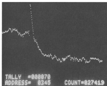
Fig. 2. Plot of light intensity at 250.5 nm vs. time after the flash in the 310.5 nm photolysis of a mixture containing \text{Cl}_2 at 3.4 Torr, \text{C}_2\text{H}_6 at about 2.5 Torr and excess \text{O}_2 to bring the total pressure to 54.0 Torr. The time scale runs from left to right with a sweep time of 2 \mu\text{s} per channel. The fraction of light absorbed is 0.0045. The plot is an average of 21 shots.
