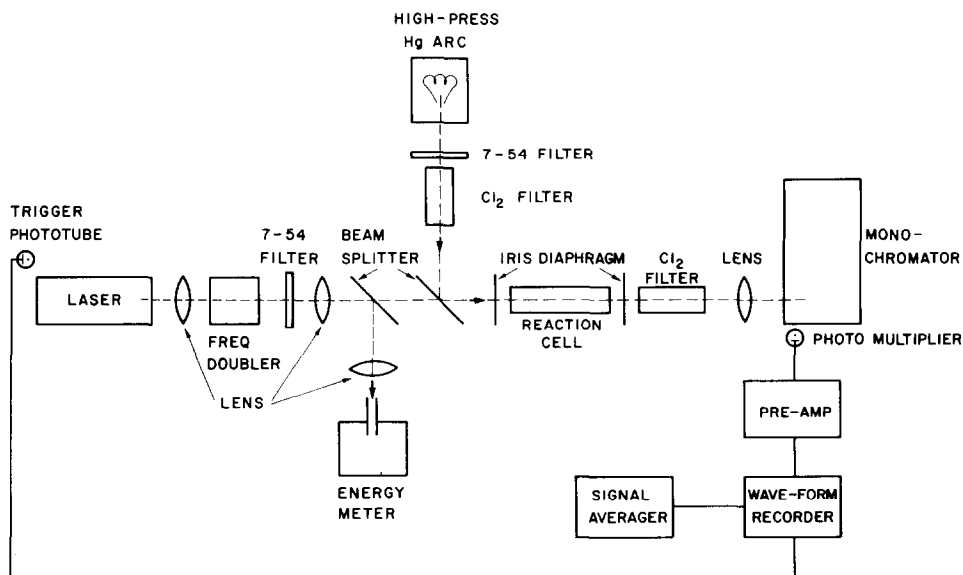
Fig. 1. Schematic diagram of the optical system.
